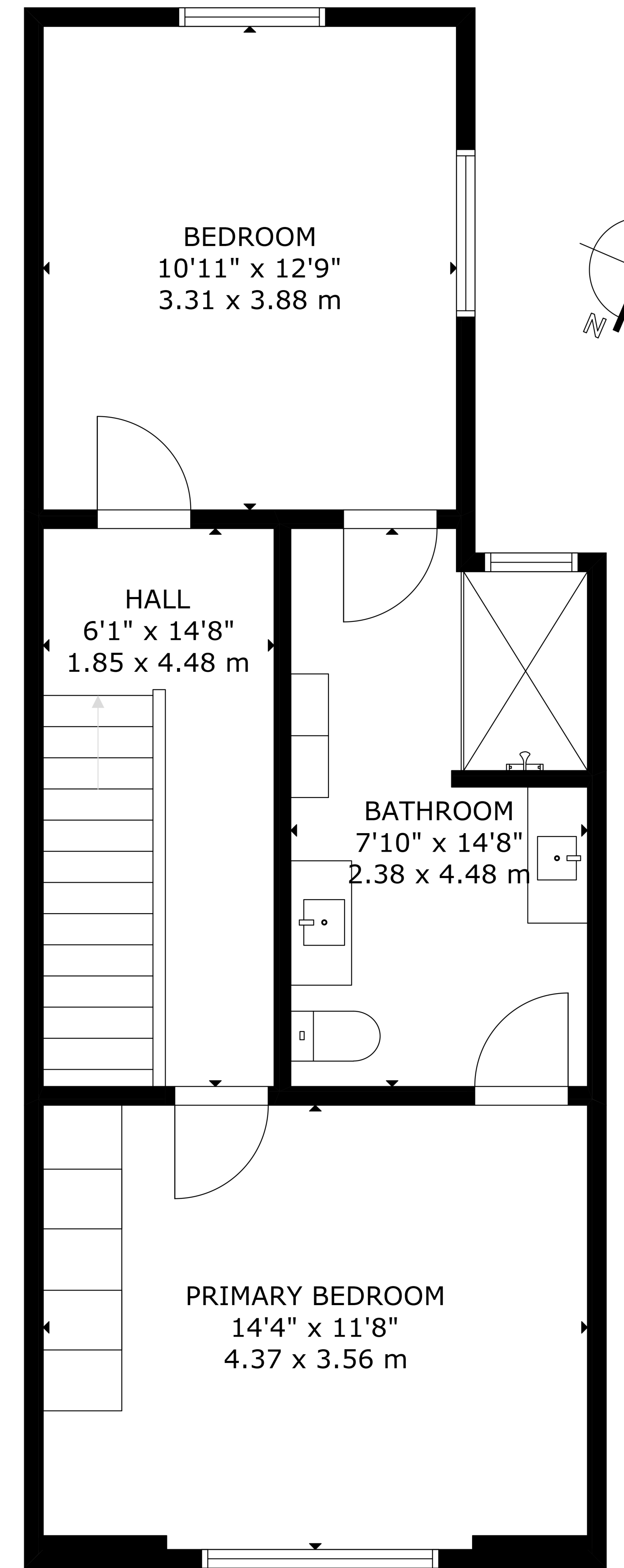
THIRD FLOOR
